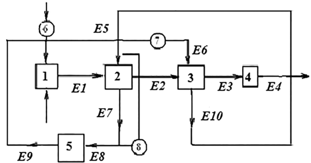
Fig. 1. Block diagram of a boiler plant with a heat recovery system for heating heating water: 1 — burner device; 2 — boiler; 3 — water heater; 4 — smoke exhauster; 5 — heat consumer; 6 — fan; 6–8 — pumps; E1–E4 — flue gases; E5 — E10 — water
