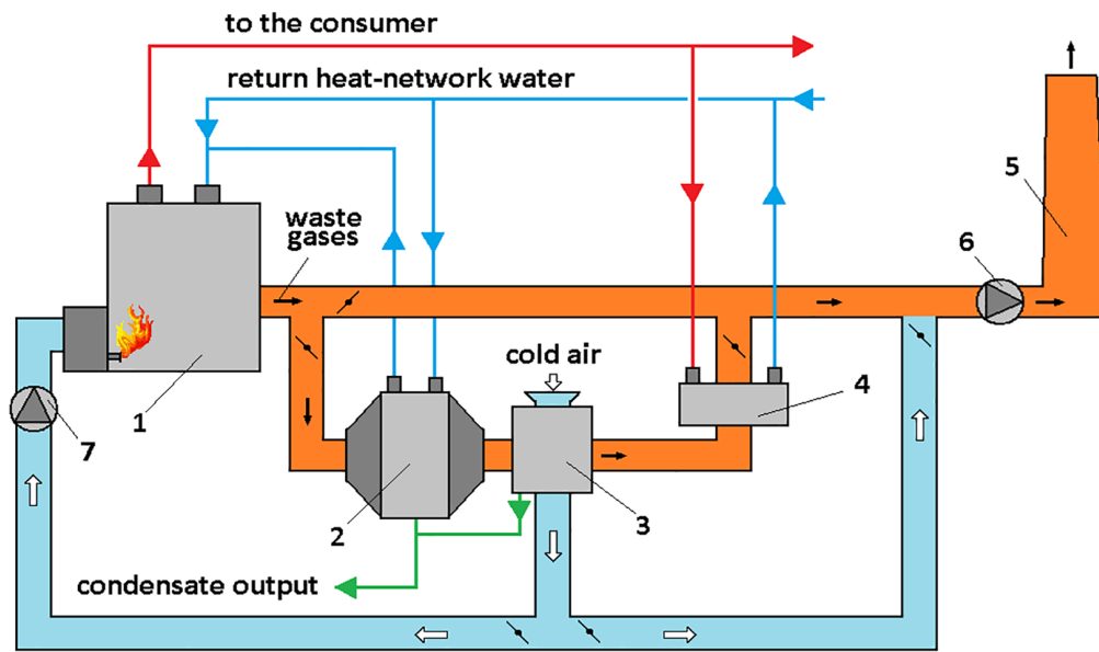
Fig. 1. Schematic circuit of the complex heat-recovery plant: 1 — boiler; 2 — water-heater; 3 — air-heater; 4 — gas-heater; 5 — chimney; 6 — exhauster; 7 — blower
